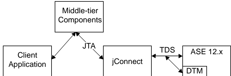
Figure 2-2: Distributed transaction management support with version 12.x
