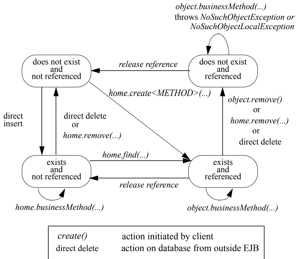
Figure 11 Client View of Entity Object Life Cycle
