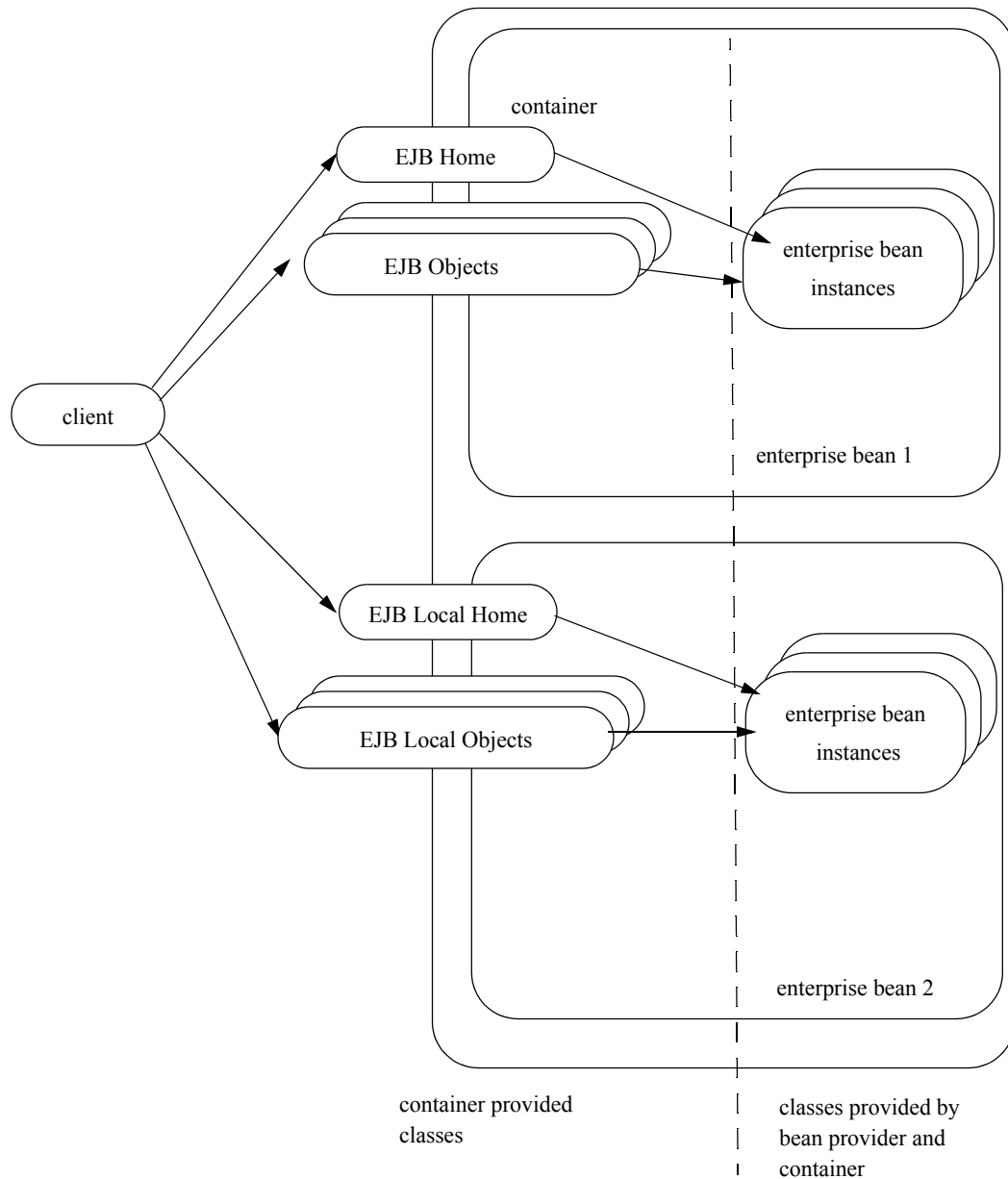
Figure 14 Overview of the Entity Bean Runtime Execution Model
