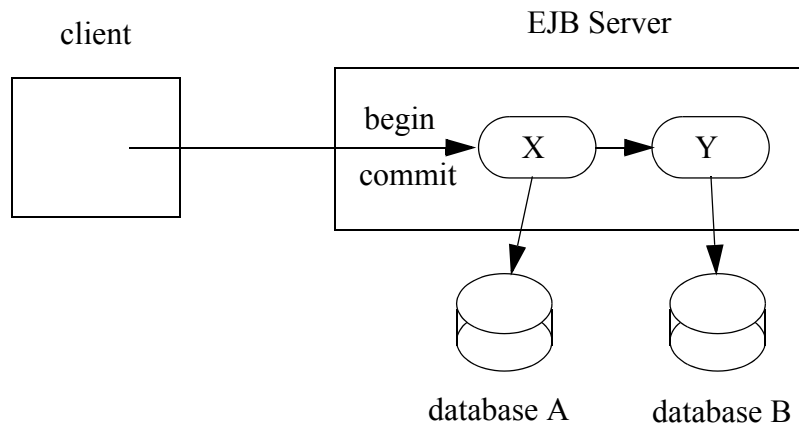
Figure 29 Update of Multiple Databases from Non-Transactional Client
