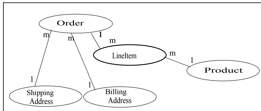
Figure 18 Several Entity Beans with Abstract Persistence Schemas Defined in the Same Ejb-jar File.
