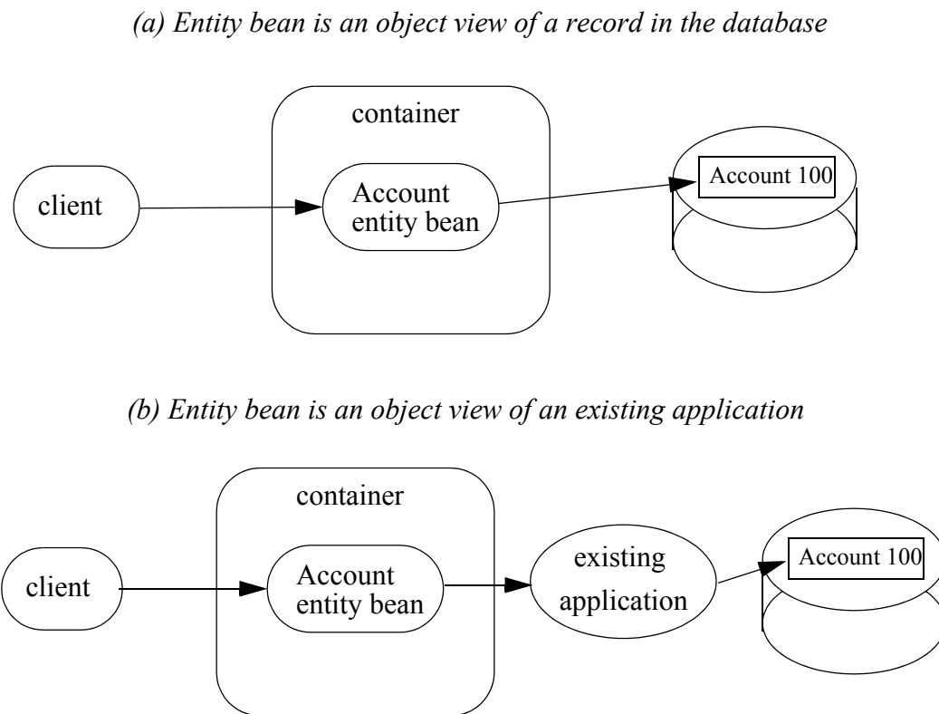
Figure 19 Client View of Underlying Data Sources Accessed Through Entity Bean
