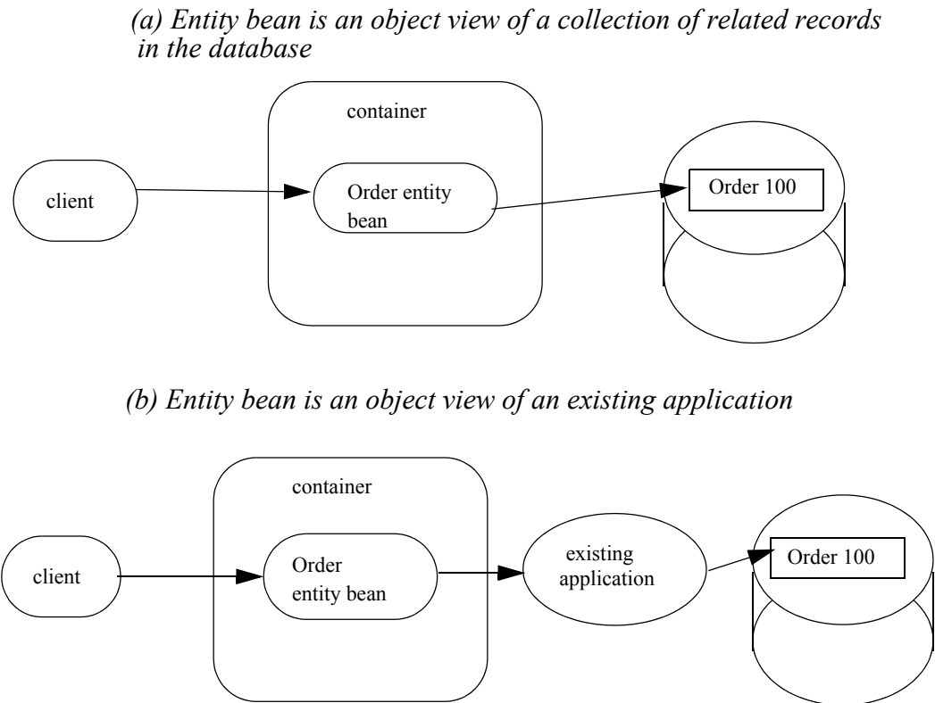
Figure 12 View of Underlying Data Sources Accessed Through Entity Bean
