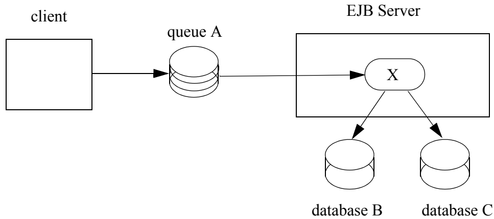
Figure 26 Message Sent to JMS Queue Serviced by Message-Driven Bean and Updates to Multiple Databases
