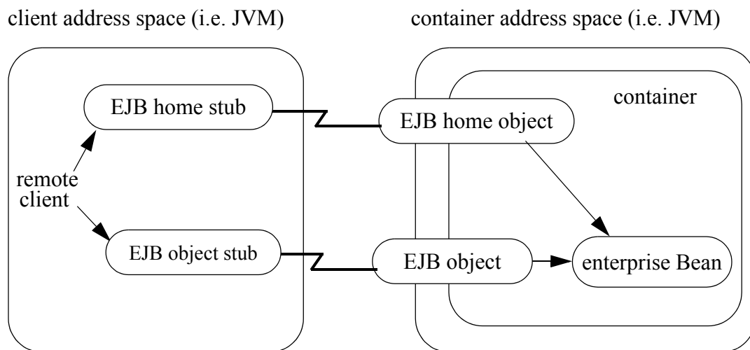
Figure 32 Location of EJB Client Stubs.
