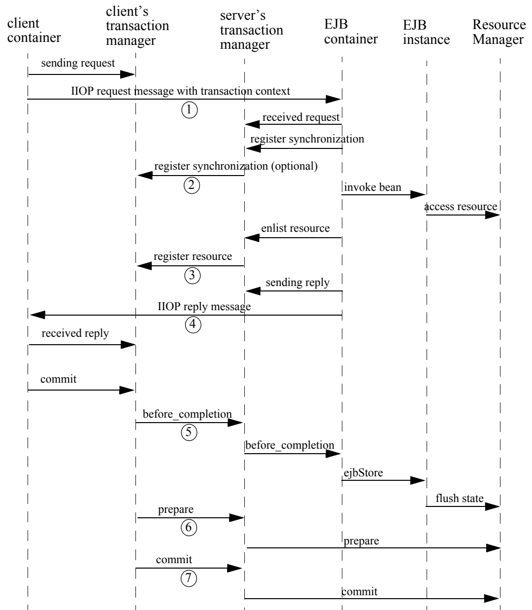
Figure 34 Transaction Context Propagation
