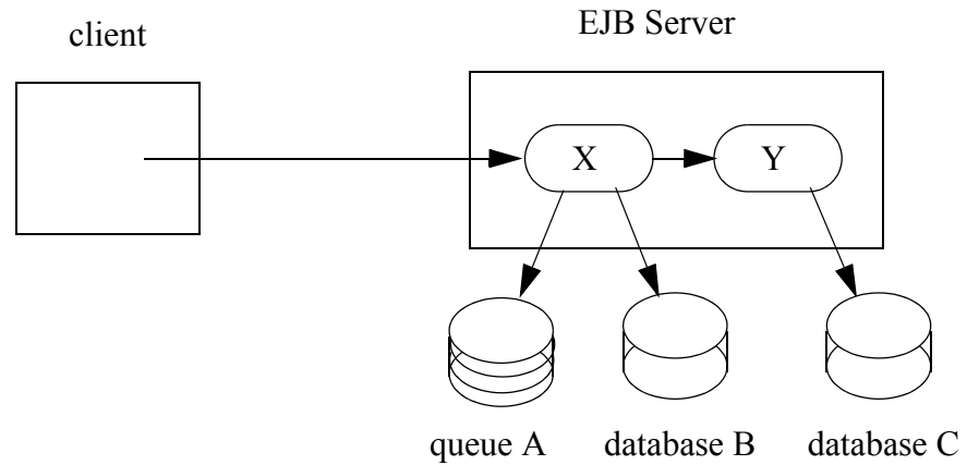
Figure 25 Message Sent to JMS Queue and Updates to Multiple Databases
