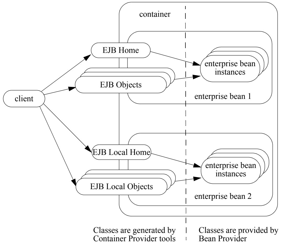
Figure 20 Overview of the Entity Bean Runtime Execution Model
