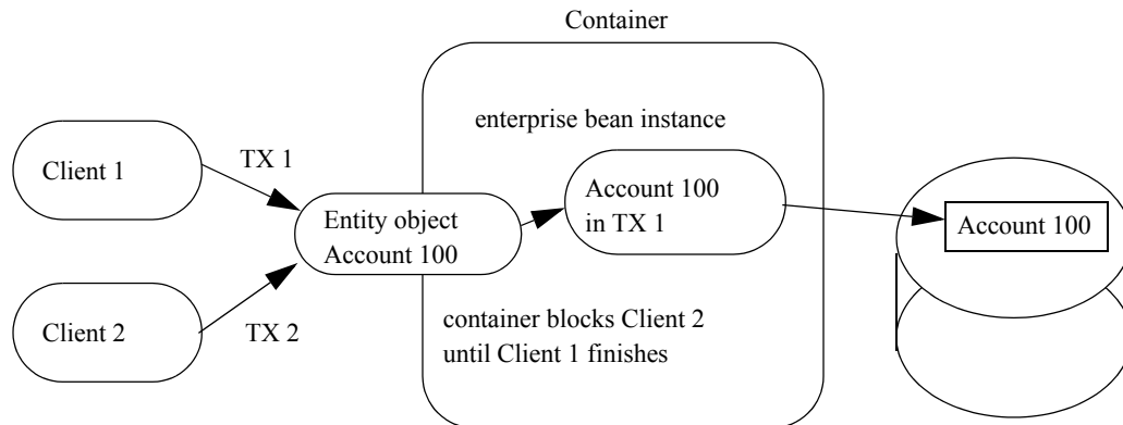
Figure 17 Multiple Clients Can Access the Same Entity Object Using Single Instance
