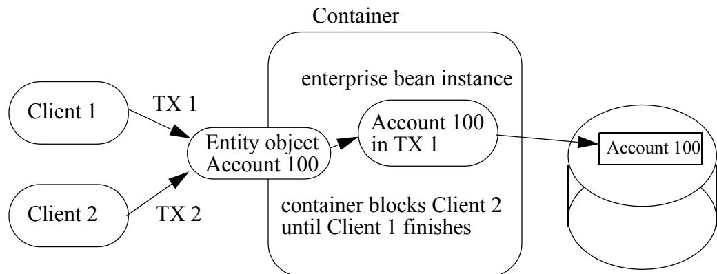
Figure 23 Multiple Clients Can Access the Same Entity Object Using Single Instance
