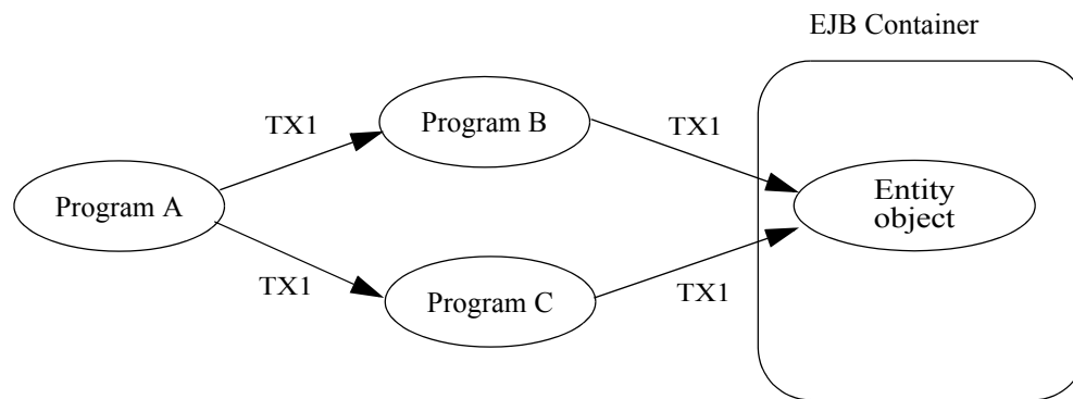
Figure 30 Transaction Diamond Scenario with Entity Object
