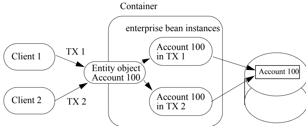
Figure 22 Multiple Clients Can Access the Same Entity Object Using Multiple Instances
