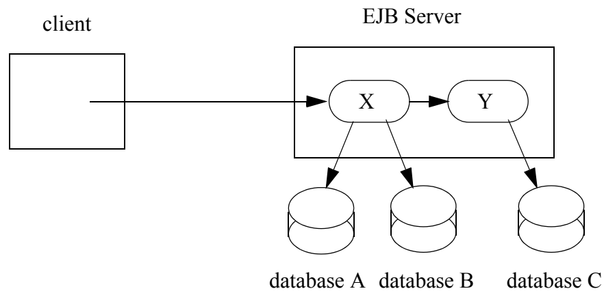
Figure 24 Updates to Simultaneous Databases
