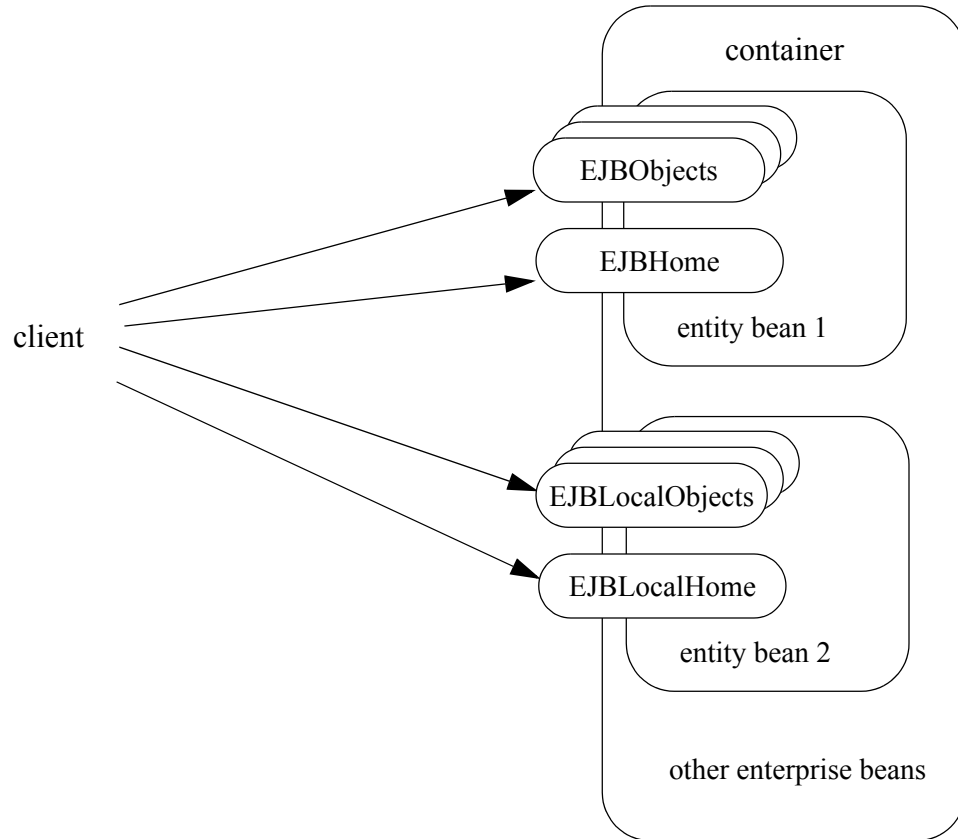
Figure 10 Client View of Entity Beans Deployed in a Container
