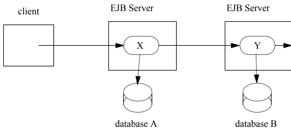
Figure 27 Updates to Multiple Databases in Same Transaction
