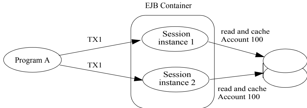
Figure 31 Transaction Diamond Scenario with a Session Bean
