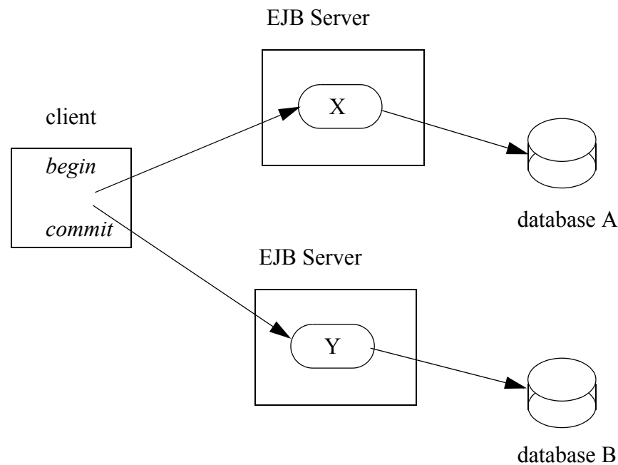
Figure 28 Updates on Multiple Databases on Multiple Servers
